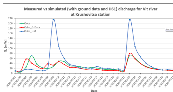
Figure 1. Simulated and observed discharges at Krushovitsa station.
