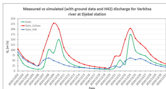
Figure 2. Simulated and observed discharges at Varbitsa station.
