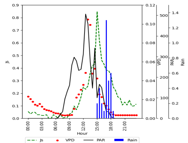
Figure 1. Diurnal dynamics of sap flow density ( J_s , \text{g m}^{-2} \text{s}^{-1} ), vapor pressure deficit (VPD, kPa), photosynthetically active radiation (PAR, \mu\text{mol m}^{-2} \text{s}^{-1} ), and precipitation (P, mm) for a representative day (29 September 2025).
