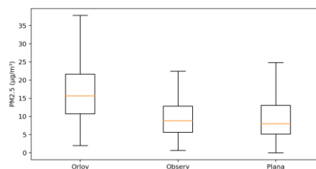
Figure 2. Distribution of hourly PM 2.5 concentrations under NW wind regime (290–340°, \geq 1 m/s).
