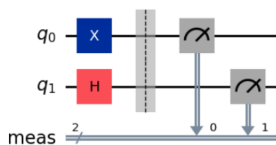
Figure 2. Simplified two-qubit quantum circuit.
