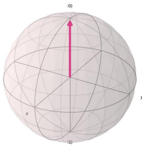
Figure 1. Visualization of the |0\rangle state of a quantum bit using the Bloch Sphere.
