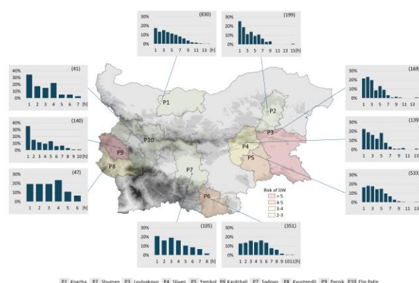
Figure 1. Relative frequency of dry winds with different durations in hours (h) at the nearest grid points to the selected stations (P1 to P10) for 1950–2025.
